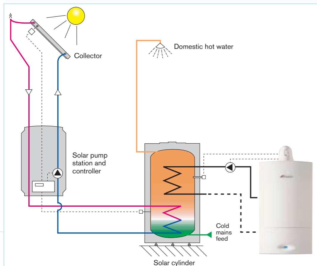
Greenskies FKC solar panel and Greenskies FKT high performance solar panels can be complemented with Greenskies twin-coil hot water cylinders with capacities of between 180 and 300 litres.
